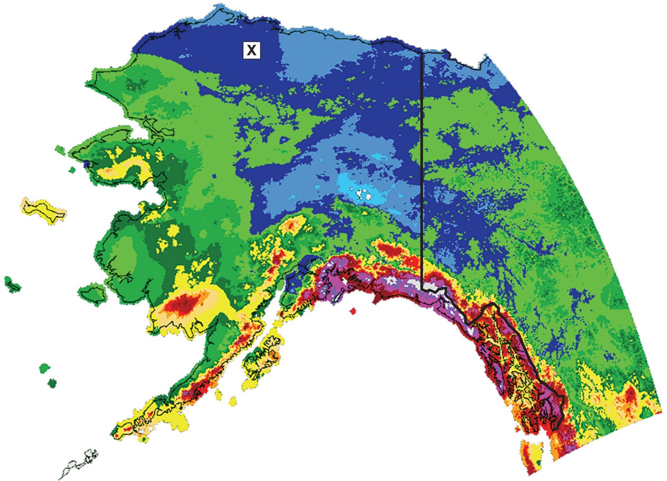
Precipitation in Alaska, USA, and part of Canada, March 2024
