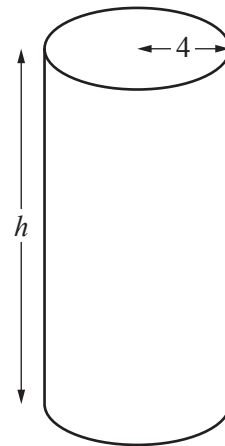
Shape I
