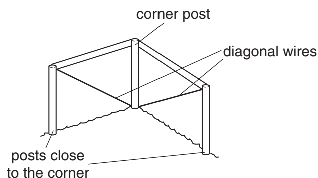
B construction of a corner
