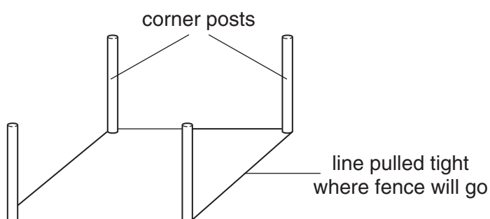
A positioning of corner posts
