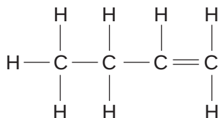
compound B
