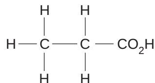
compound C
