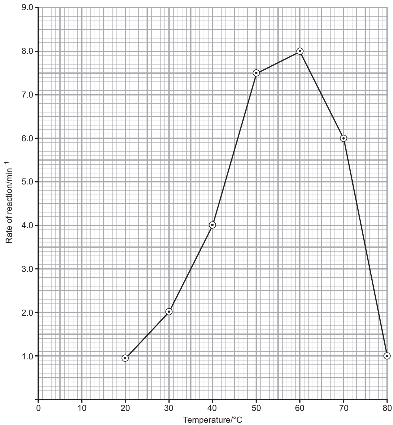
The effect of increasing temperature on the rate of reaction of a protease enzyme
