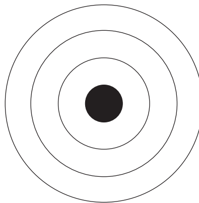
sulfur atom
