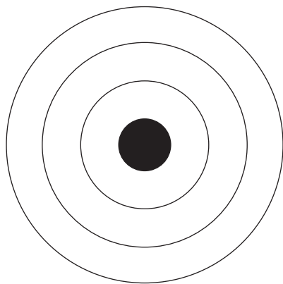
magnesium atom
