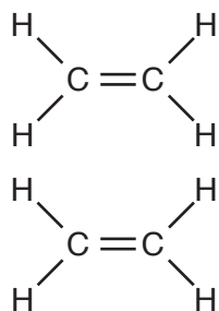
ethene
