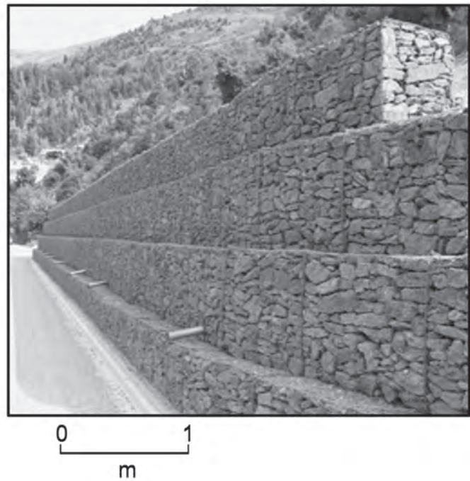
Figure 21 - stone-filled baskets (gabions)
