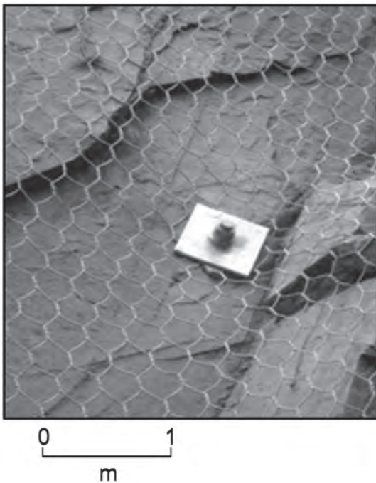
Figure 20 - rock bolts and wire netting
